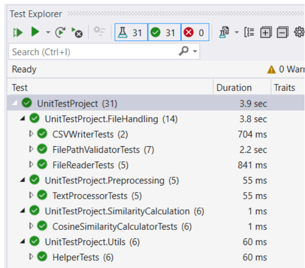
Fig 17: Unit Tests
